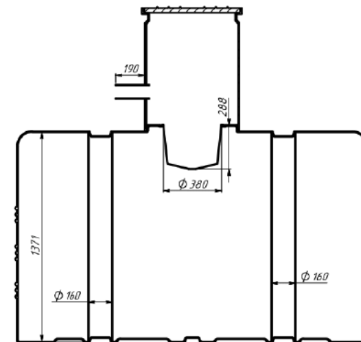
CROSS-SECTION B-B SCALE 1:12
