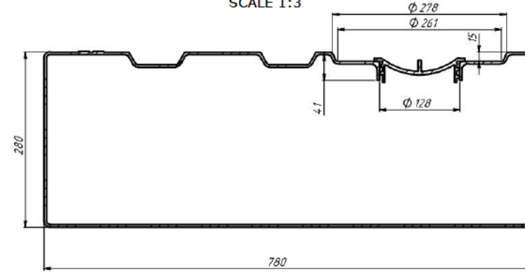
CROSS-SECTION A-A SCALE 1:3
