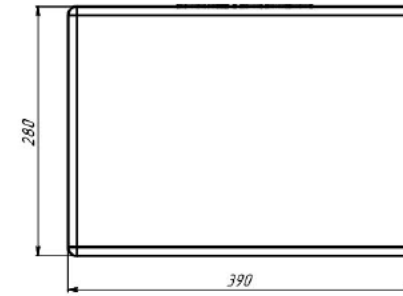
CROSS-SECTION A-A SCALE 1:3
