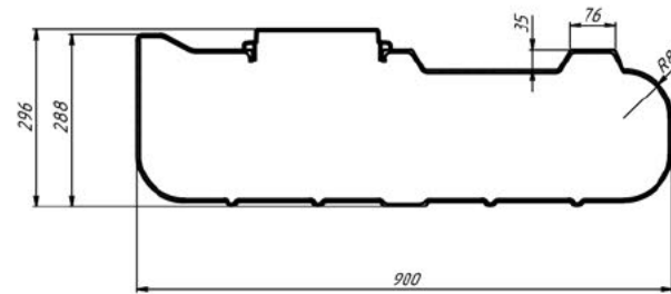
CROSS-SECTION A-A
