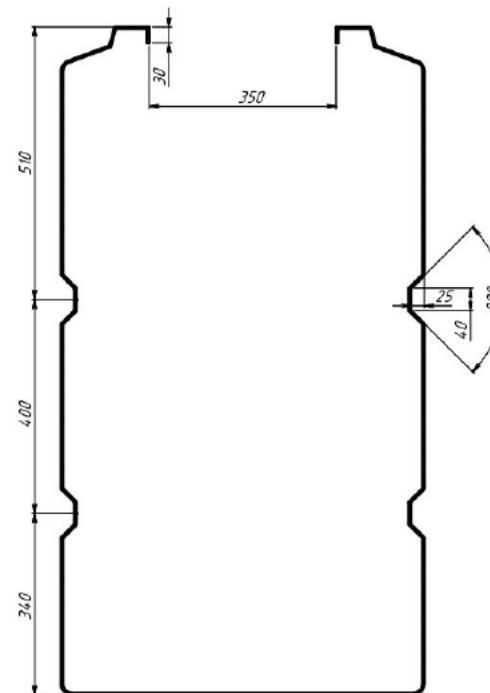
CROSS-SECTION A-A SCALE 1:5
